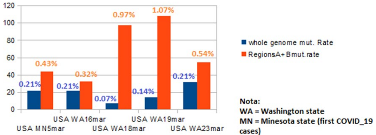
Figure 7: Comparative time evolution in WA / Minnesota regions “A” and “B”. This chart represents (WA and Minnesota strains first mutations) and mutations/deletions rates % at whole genome and in the case of region 930 bases = region « A » (600bases) + region « B » (330 bases).
